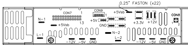
Rear View
